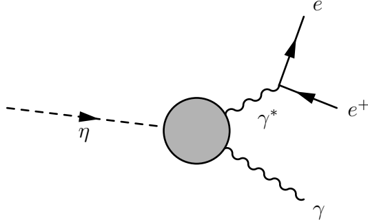
Figure A.3: Diagram of Dalitz decay of \eta meson.
