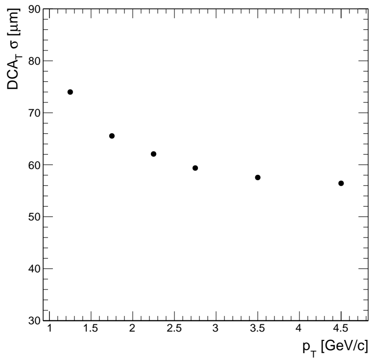
Figure 5.8: The DCA T resolution as a function of p_T for all tracks in MB events
