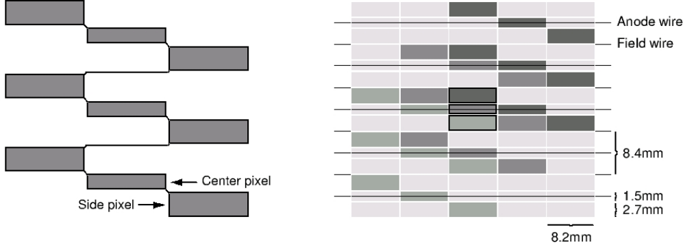
Figure 4.7: The pad and pixel geometry in the pad chamber. A cell defined by three pixels is at the center of the right picture.
