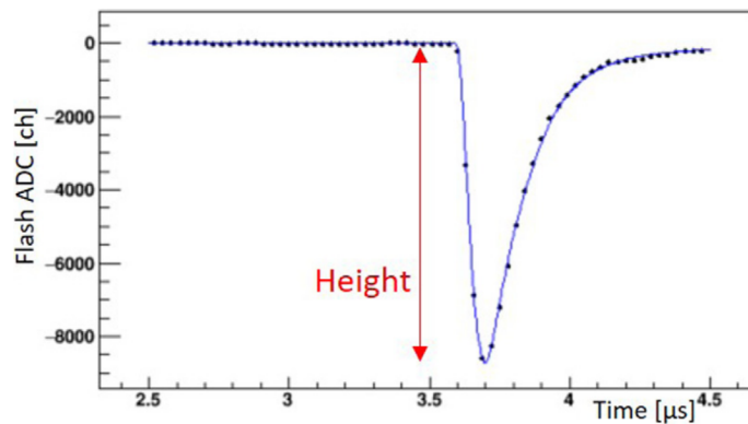
Figure 2.22: Typical waveform of the BGO calorimeter after the shaping circuit [39]. The black points show the flash ADC data with a sampling rate of 33 MHz. The blue line shows the reconstructed pulse shape by fitting the data point with a template waveform.
