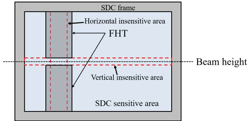
Figure 4.6: Rough sketch of insensitve region in SDC2 or SDC3. The area surrounded by red dotted lines indicates insensitve region of SDC and the beam particles passed through around the center of cross-shape, where SDCs were completely insensitve. Although the horizontal insensitve areas were covered by FHT, the vertical insensitve areas could not be recovered.
