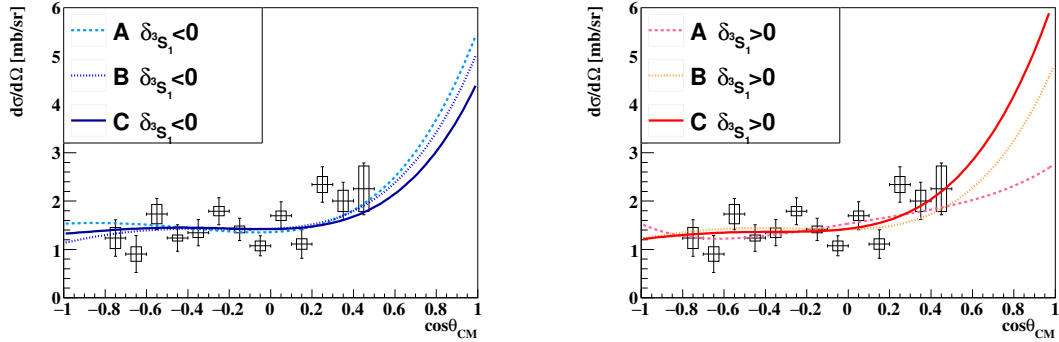
Figure 7.3: Differential cross section as a function of the scattering angle together with the calculated angular distribution in the phase-shift analysis for the middle-momentum region ( 0.55 < p_{\Sigma}[\text{GeV}/c] < 0.65 ). The fitting conditions are the same as in Figure 7.2. The typical \chi^2/\text{ndf} is 14.0/11.
