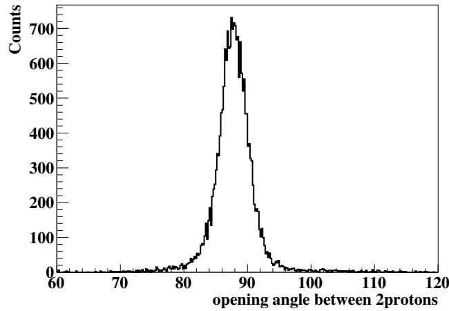
Figure 4.22: Opening angle between two protons for pp scattering with the beam momentum of 0.6 GeV/c.
