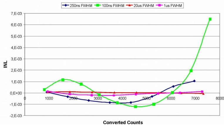
INL for different shaping times
