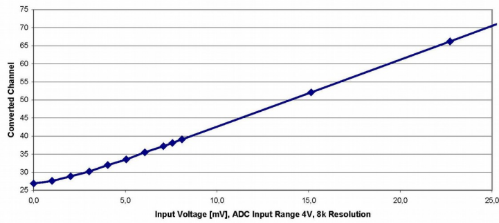
INL at 20us FWHM
