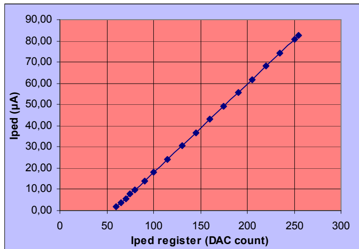
Fig. 2.6: Iped (μA) Vs IPED-Register setting
