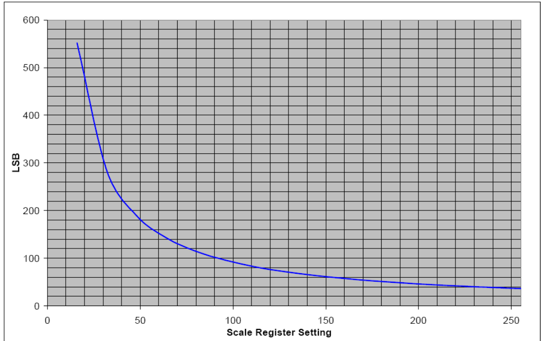
Fig. 4.33: LSB Vs. Full Scale Range Register setting
