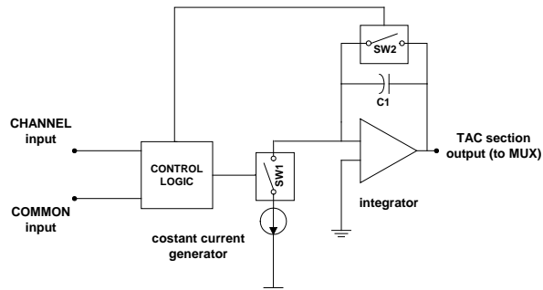
Fig. 2.1: Simplified block diagram of the TAC section
