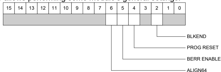
Fig. 4.19: Control Register 1
