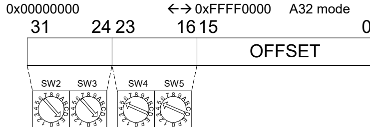
Fig. 4.2: A32 addressing
