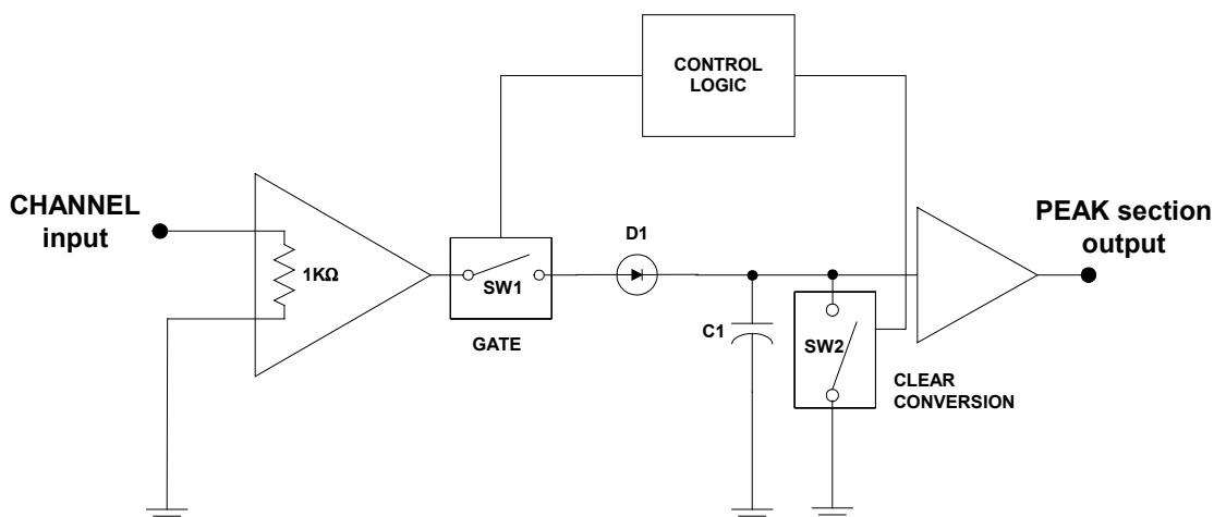
Fig. 2.1: Simplified block diagram of the PEAK section
