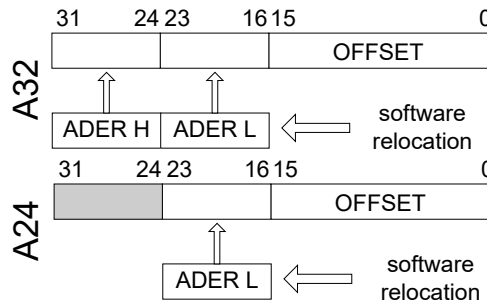
Fig. 4.4: Software relocation of base address
