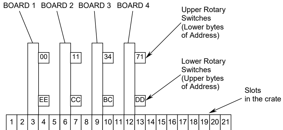
Fig. 4.6: MCST/CBLT Addressing Example
