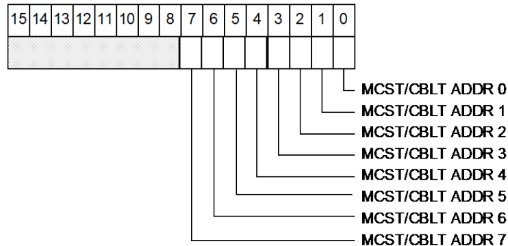
Fig. 4.14: MCST/CBLT address register
