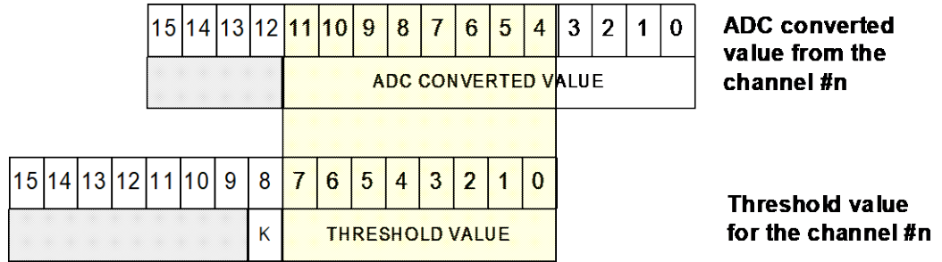
Fig. 2.5: Zero suppression (Bit 8 of Bit Set 2 Register = 0, default setting)
