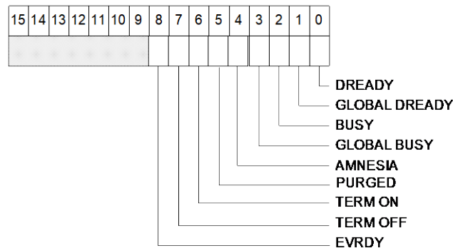
Fig. 4.18: Status Register 1
