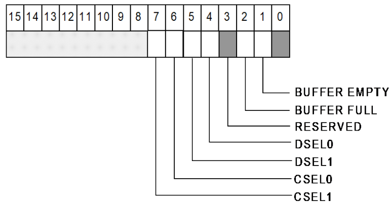
Fig. 4.24: Status Register 2
