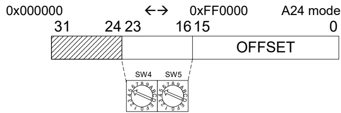
Fig. 4.1: A24 addressing
