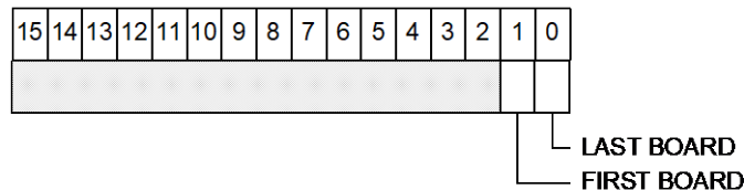
Fig. 4.22: MCST Address Register
