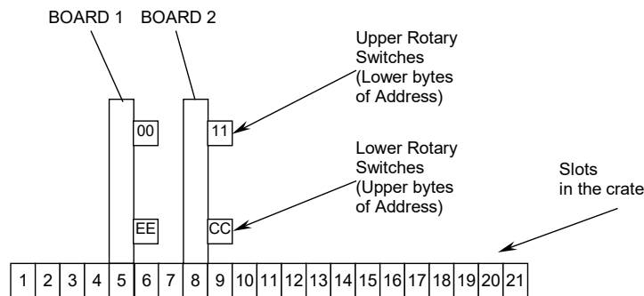
Fig. 4.5: Base/GEO Addressing: Example 1
