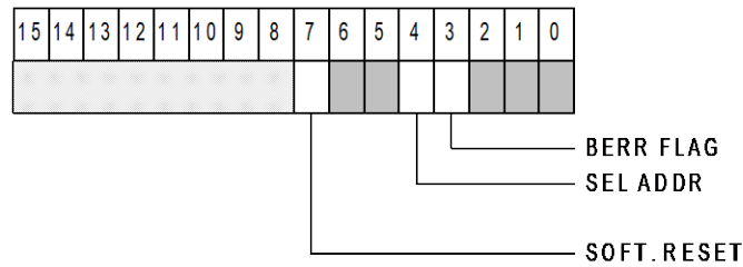
Fig. 4.15: Bit Set 1 Register
