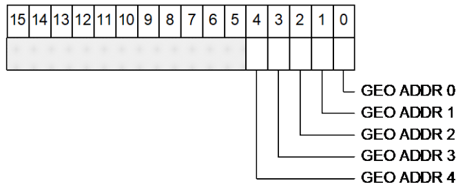
Fig. 4.13: Geographical address register
